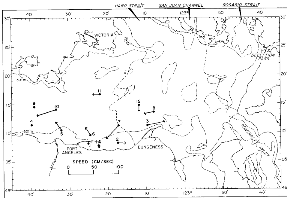
Figure 3.2. Plan view of mean currents near the surface (approximately 5 m depth) from longer period current meter records. Dots without arrows lack current meters at 5 m depth. Site numbers correspond to data shown in Appendix A.2. Notation: dashed lines, selected sills.
