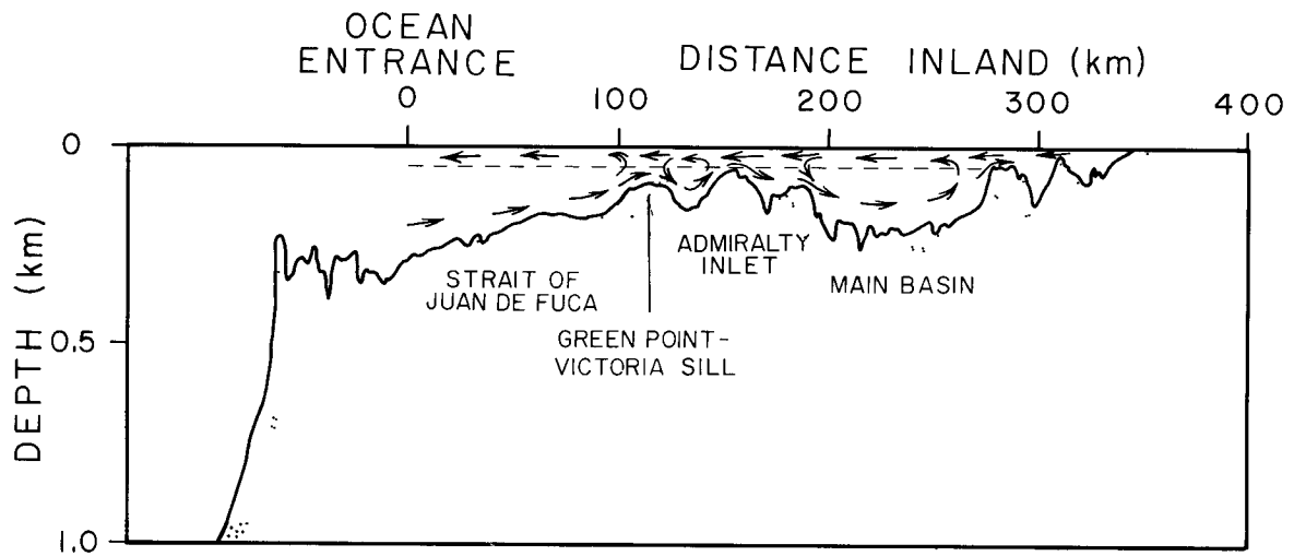
Figure 3.1. Profile view of net circulation at mid-channel in summer between the Pacific Ocean and the head of Puget Sound (adapted from Ebbesmeyer and Barnes, 1979) Notation: dashed line, depth of no-net-motion (approximately 50 m).
