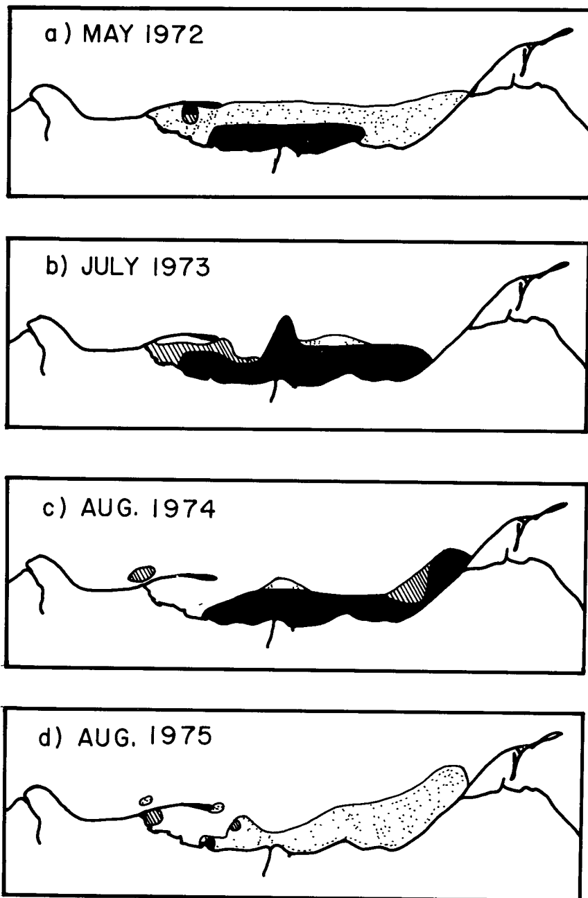
Figure 5.5. Oyster larvae bioassay tests of effluent toxicity on four occasions (a-d; from Cardwell et al. , 1977). Notation: stippled, greater than 5% abnormality; hatched, greater than 20% abnormality; and blackened, greater than 50% abnormality.
