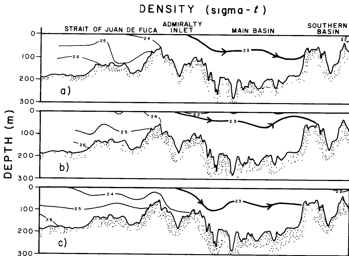
Figure 5.13. Profile view of density (expressed in sigma-t units) at mid-channel from the inner Strait of Juan de Fuca to Puget Sound's Main Basin (adapted from Collias et al. , 1974). Heavy lines with arrowheads denote possible pathway at depth of oil transport into Puget Sound. Dates: a) 15-17 September 1958, b) 19-21 November 1958; and c) 19-23 December 1958.
