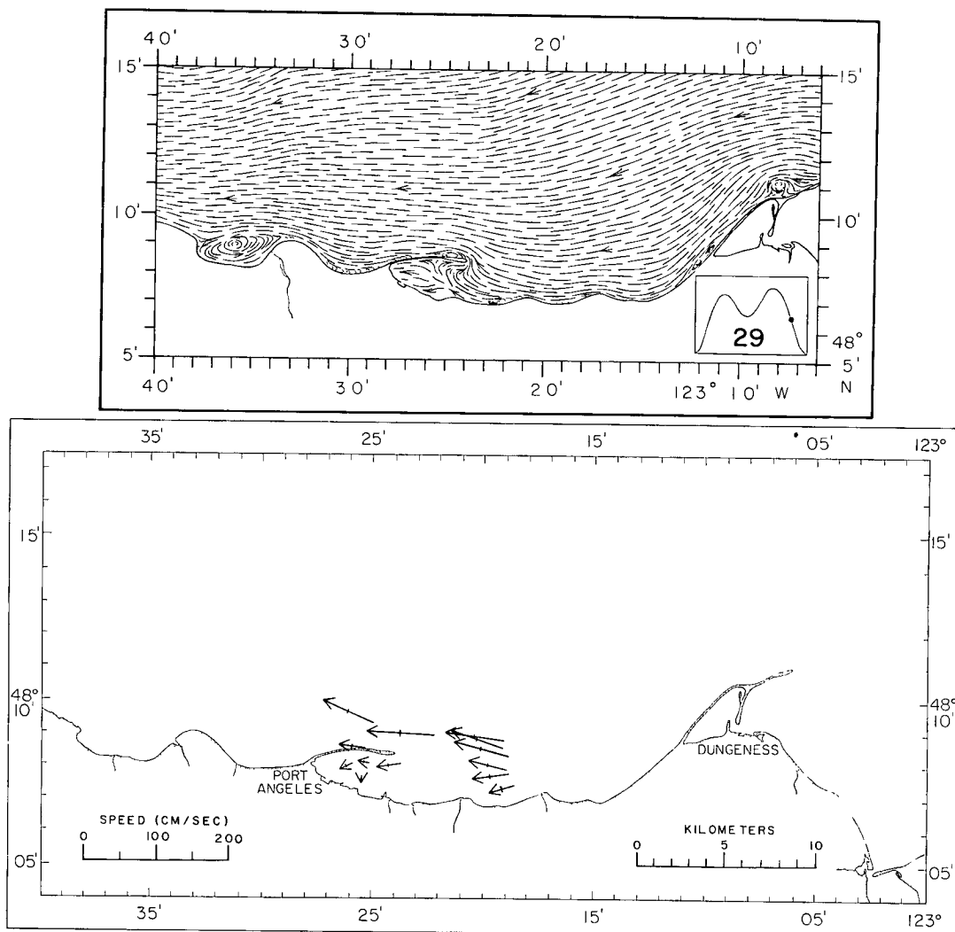
Appendix D.11. Top: Tidal current pattern from hydraulic tidal model. Inset shows tidal phase. Bottom: Drift sheet spatial vector diagram at 0900 24 April 1978 from Ebbesmeyer et al. (1978).
