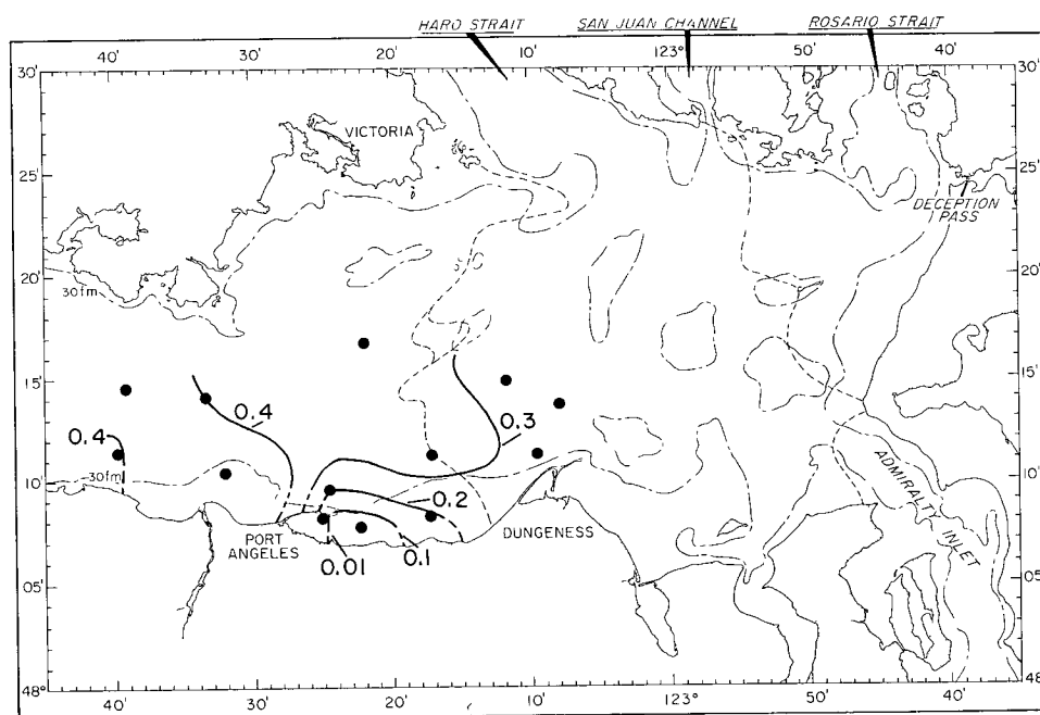
Figure 3.3. Plan view of variance near the surface (approximately 5 m depth) of longer period current meter records. Note change in contour interval between 0.1 and 0.01 \text{m}^2 \text{s}^{-2} . Notation: dashed lines, selected sills.
