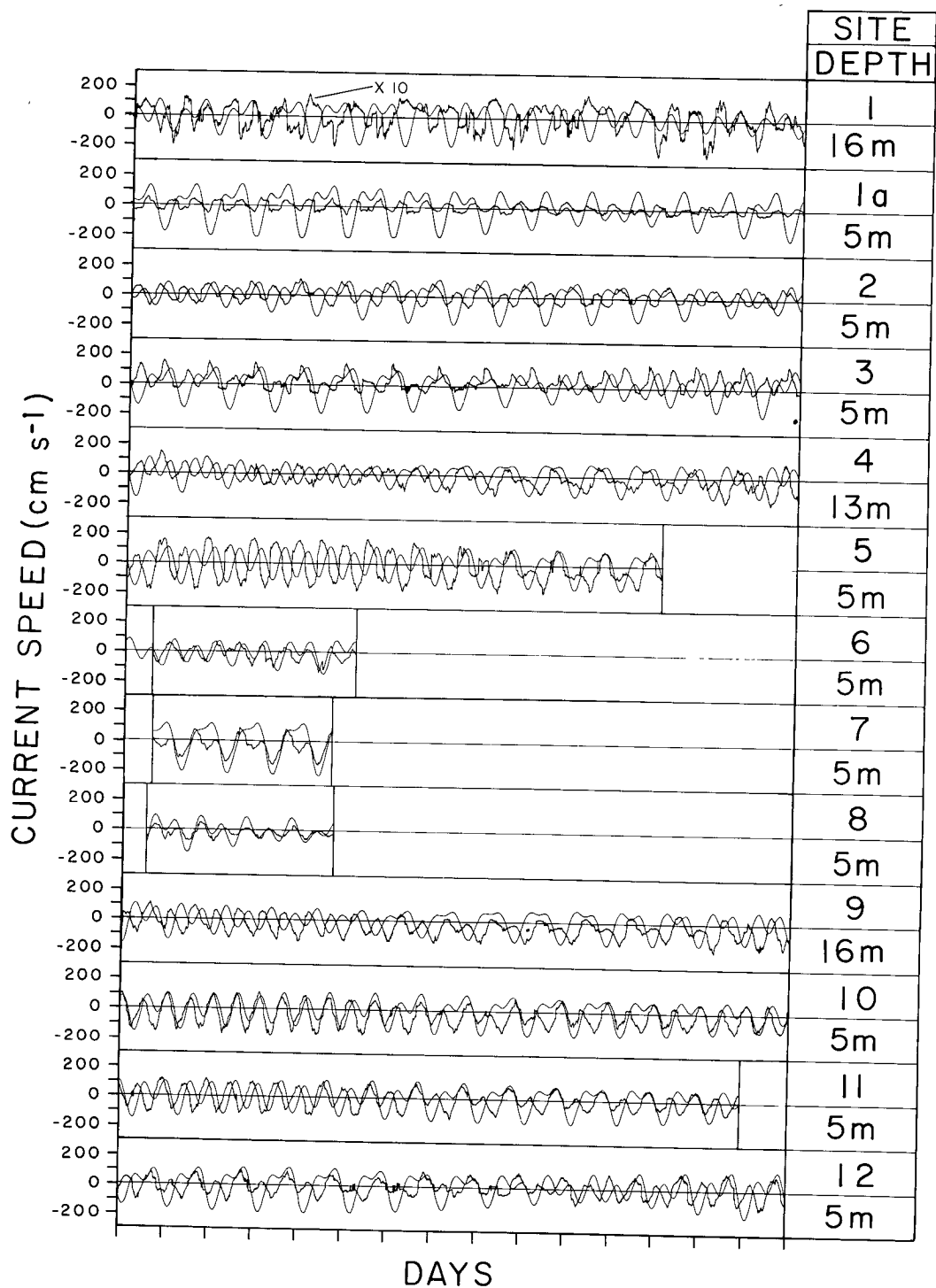
Figure 3.4. Time series of longer period current meter records. Sites of current meter moorings are shown in Figure 3.2 and listed in Appendix A.2. Smooth lines represent predicted tides at Port Angeles and other lines are observed current speeds where positive and negative are reckoned toward the east ( 001-180^{\circ} True) and west ( 181-360^{\circ} True), respectively.
