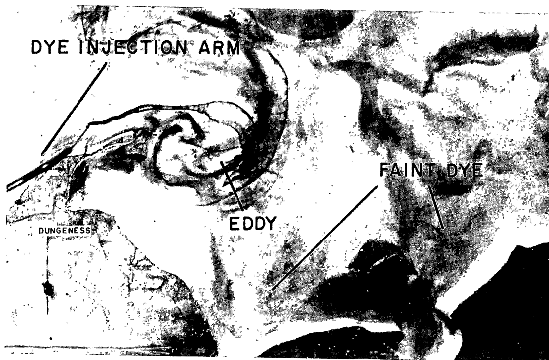
Figure 5.11 Streak photographs of a tidal eddy in the lee of Dungeness Spit in the hydraulic tidal model. Dot on inset shows tidal phase of streak photograph.
